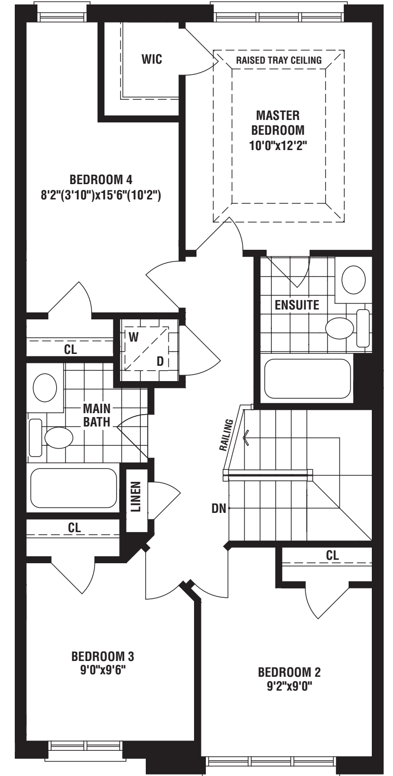
OPT. UPPER FLOOR PLAN ELEV. 'A' (4 BEDROOM)
