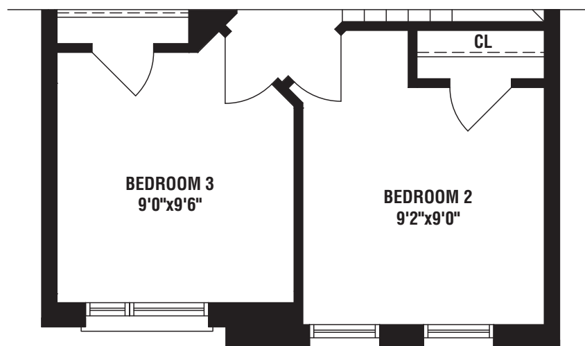
PARTIAL UPPER FLOOR PLAN ELEV. 'B' (3 & 4 BEDROOM)
