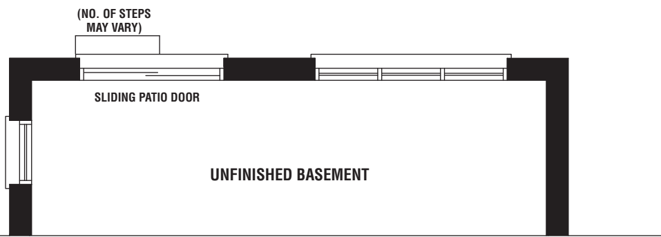
PARTIAL BASEMENT PLAN W.O.B. CONDITION
