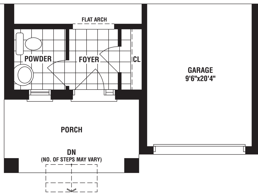
PARTIAL GROUND FLOOR PLAN ELEV. 'B'
