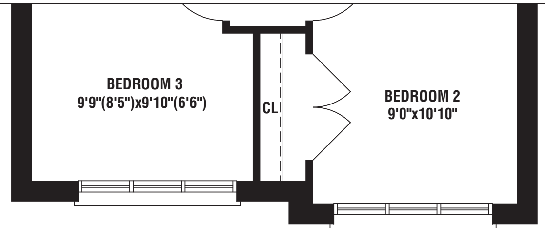
PARTIAL SECOND FLOOR PLAN ELEV. 'B'
