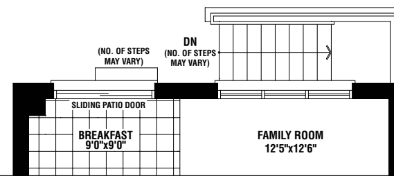
PARTIAL OPT. GROUND FLOOR PLAN WALK-UP CONDITION
