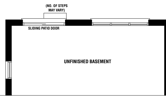
PARTIAL BASEMENT PLAN W.O.B. CONDITION
