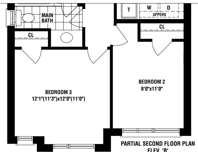
PARTIAL OPT. SECOND FLOOR PLAN ELEV. 'B' (4 BEDROOM)
