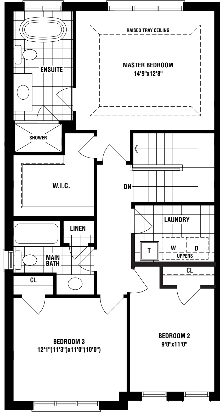
SECOND FLOOR PLAN ELEV. 'A' (3 BEDROOM)
