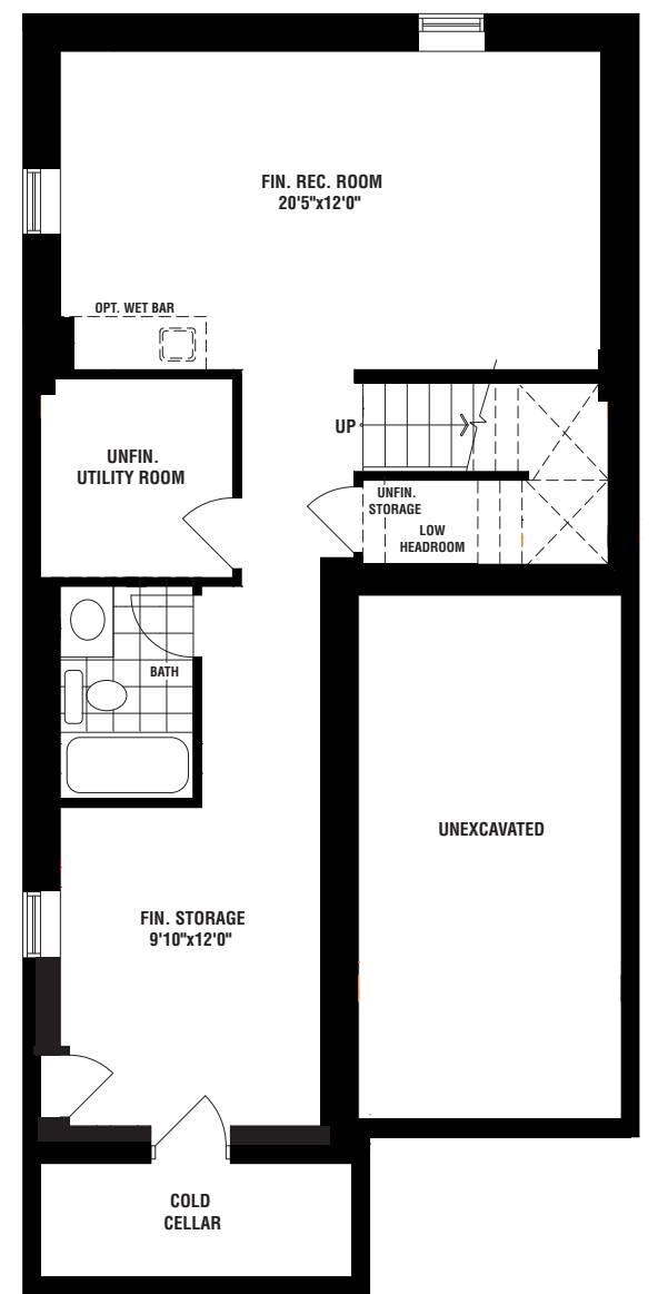
OPT. FINISHED BASEMENT PLAN ELEV. 'A'
