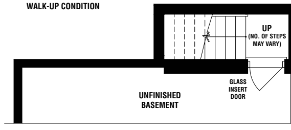
PARTIAL OPT. BASEMENT PLAN WALK-UP CONDITION
