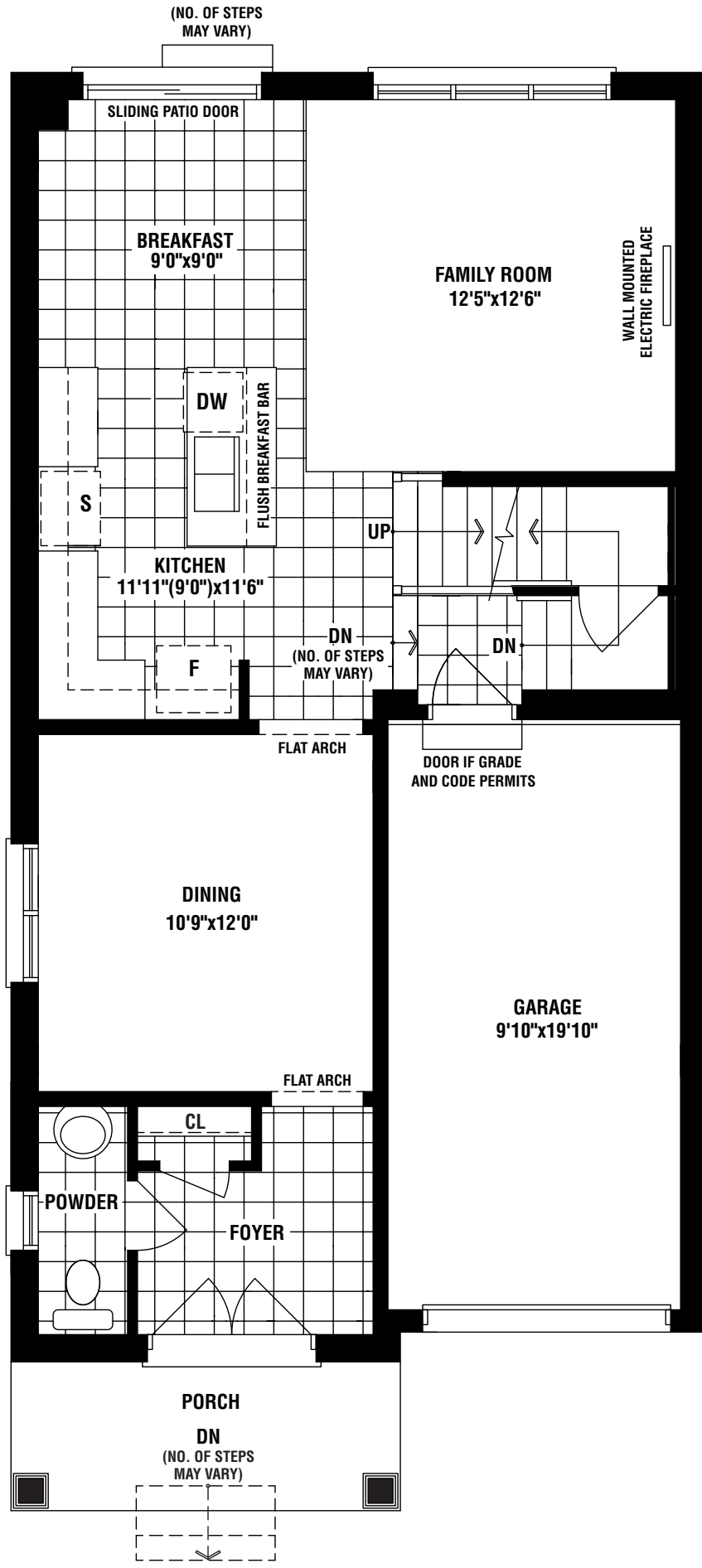
GROUND FLOOR PLAN ELEV. 'A'
