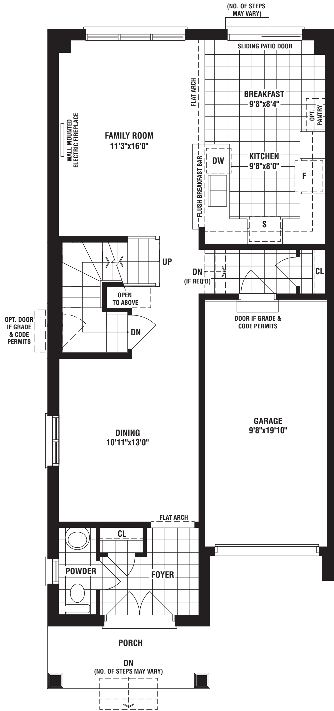
GROUND FLOOR PLAN ELEV. 'A'
