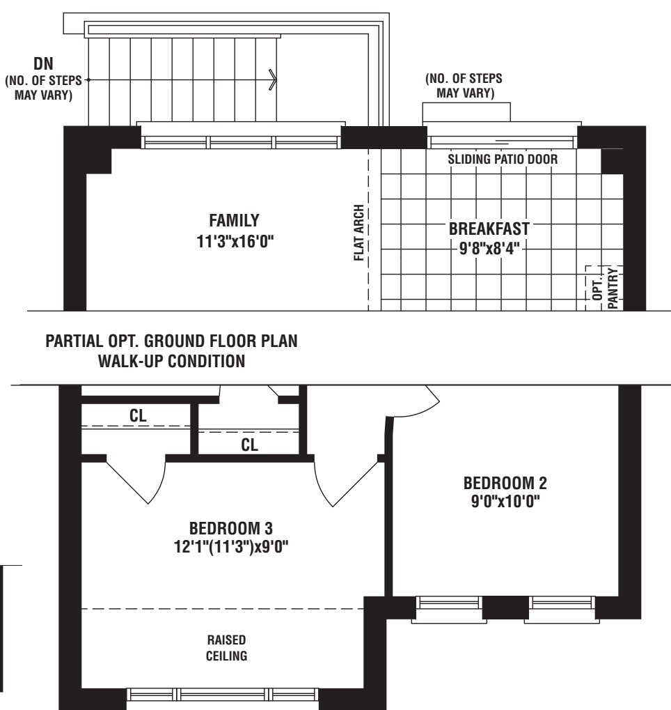
PARTIAL SECOND FLOOR PLAN ELEV. 'B'
