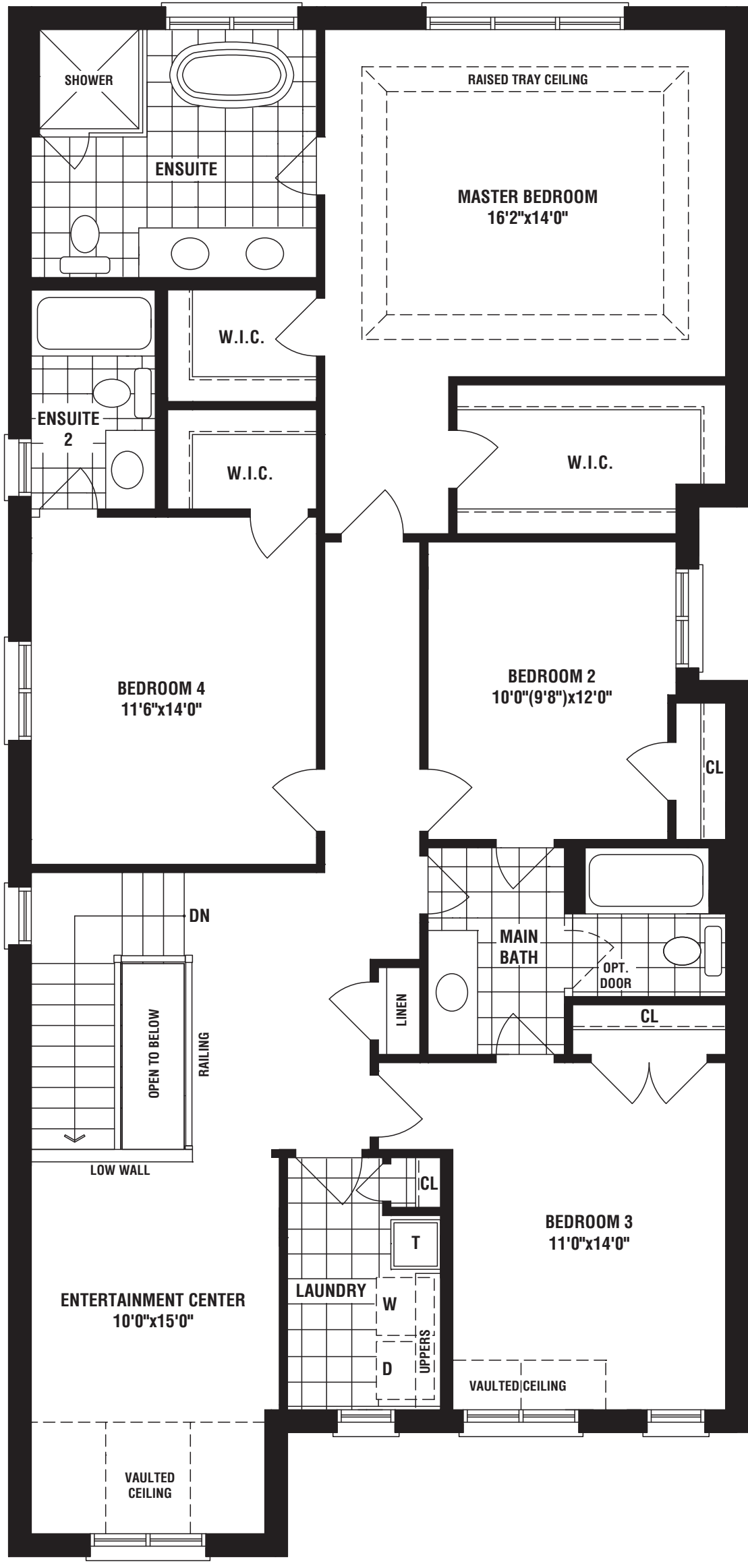
SECOND FLOOR PLAN ELEV. 'A' (4 BEDROOM)
