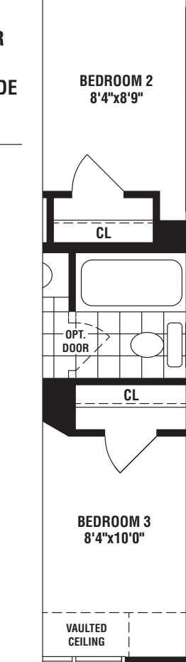
PARTIAL OPT. UPPER FLOOR PLAN ELEV. 'A' UPGRADE (4 BEDROOM)
