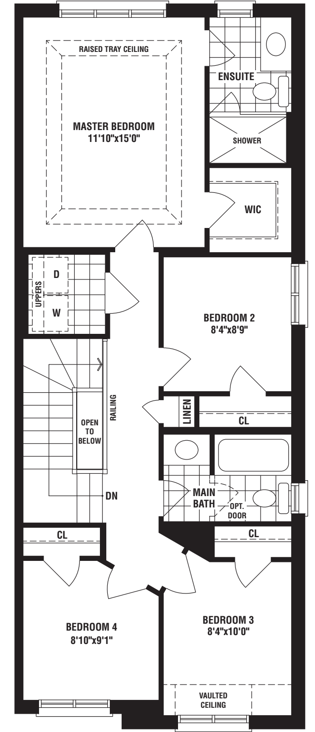
OPT. UPPER FLOOR PLAN ELEV. 'A' (4 BEDROOM)
