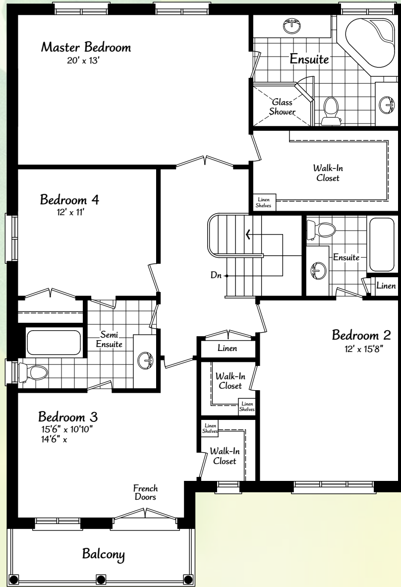
Second Floor Plan 'A'
